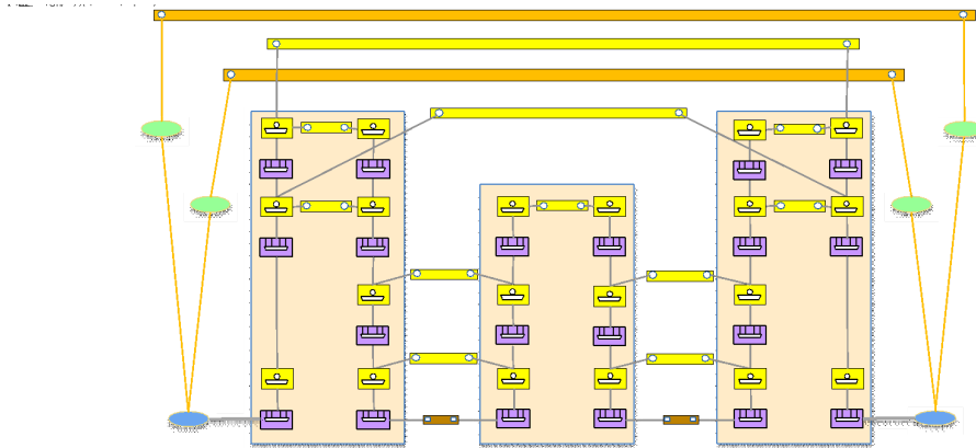
Figure 5-9 Scenario 1 : Optical Line System Controller, MC and OTSiMC CSs
