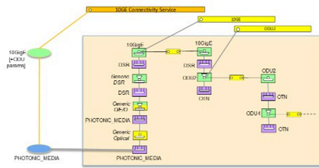
Figure 5-43 DSR UNI, explicit model of functions (optical)
