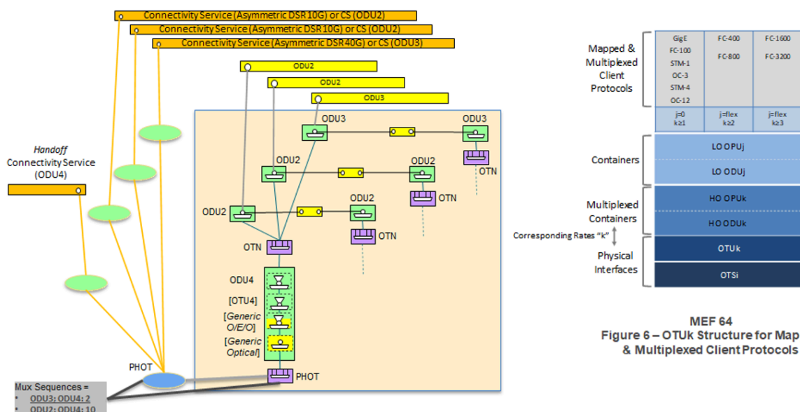
Figure 5-50 OTN ENNI, mapped & multiplexed client protocols, with additional embedded functions
