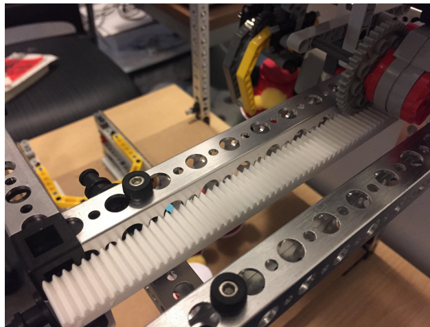
Figure 1.1: 3D printed gear track and motor drive system
