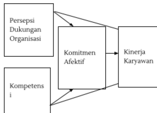
Figure 1. Research Model
