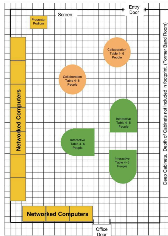
General floorplan by Melissa Oliver, Used with Permission and adapted for project
