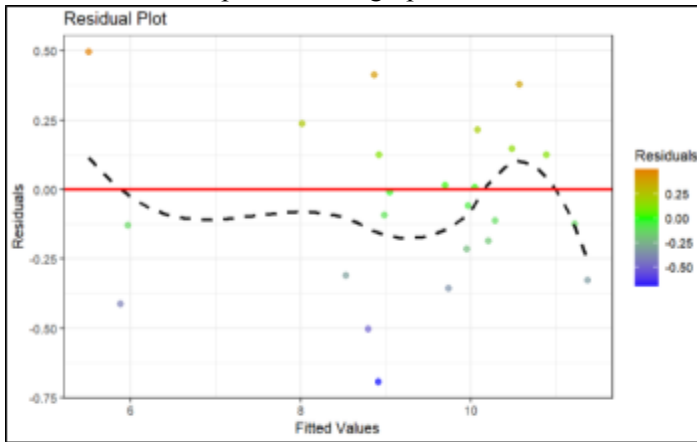
Figure 6: MARS residuals against fitted values
