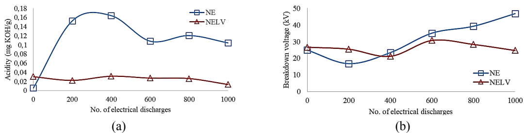
Figure 2. Effects of electrical discharges to (a) acidity of HVNE and NELV and (b) breakdown voltage of NE and NELV samples
