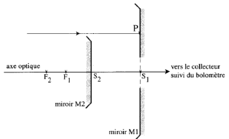
Figure 5 - Antenne Cassegrain
