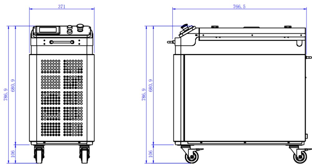
Figure 2.3 Dimensional diagram of GY-FLC500S laser cleaning machine
