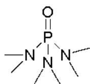
HMPA
