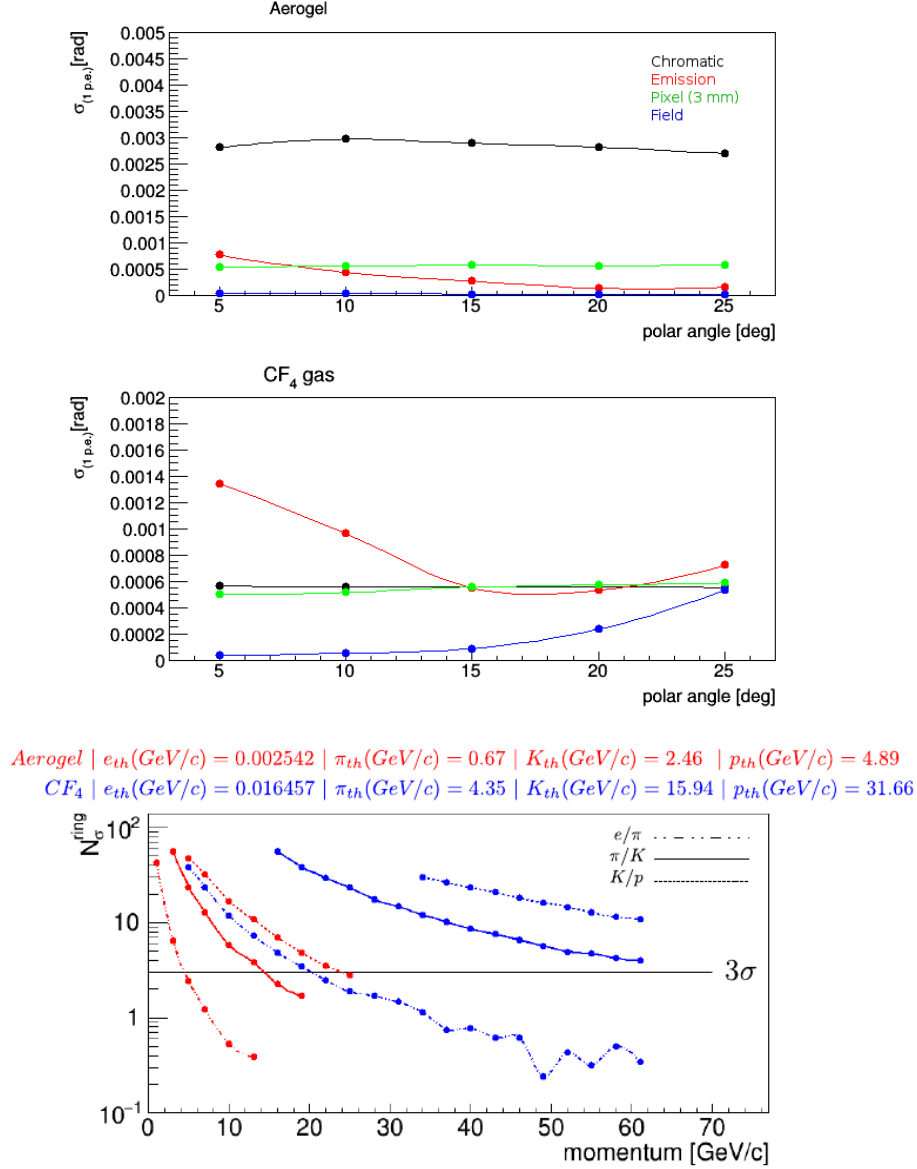
Figure 2.2.2 (upper panel) Single p.e. error sources, for a 30 GeV/c pion, assuming a pixel size of 3 mm. (lower panel) Particle separation power for tracks with 15° polar angle, using \text{CF}_4 as a gas radiator (see Figure 2.1.4 for \text{C}_2\text{F}_6 ).
