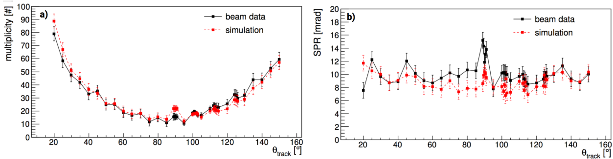
Figure 2.4.4: Results from the 2015 CERN beam test: Photon yield (a) and SPR (b) as a function of the track polar angle for the narrow bar and the 3-layer spherical lens for tagged protons at 7 \text{ GeV}/c beam momentum in data (black) and Geant simulation (red). The error bars correspond to the rms of the distribution in each bin.
