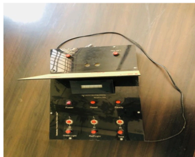
Reaction Time Apparatus
