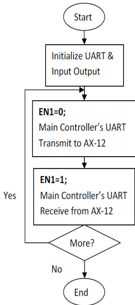
AX-12 Serial Communication Flow
