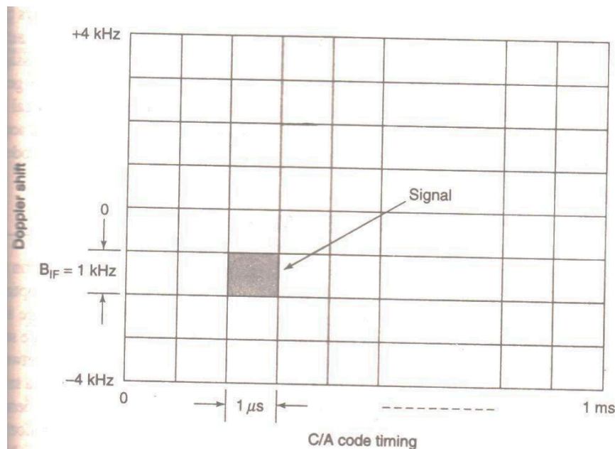
FIGURE -Code synchronization and doppler tracking matrix
