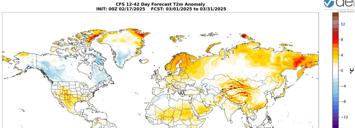
Figure 15. Forecasted average surface temperature anomalies ( ^{\circ}\text{C} ; shading) across the Northern Hemisphere for March 2025. The forecasts are from the CFS 00Z 17 February 2025.
