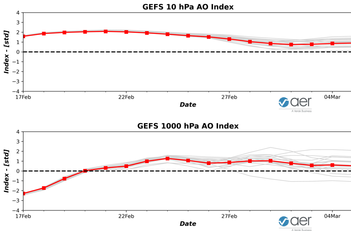
Figure 1. a) The predicted daily-mean AO at 10 hPa from the 00Z 17 February 2025 GFS ensemble. b) The predicted daily-mean AO at 1000 hPa from the 00Z 17 February 2025 GFS ensemble. Gray lines indicate the AO index from each individual ensemble member, with the ensemble mean AO index given by the red line with squares.
