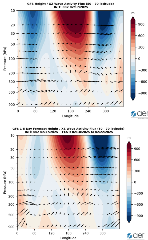
Figure iii. Longitude-height cross section of geopotential eddy height anomalies (shading) and wave activity flux (vectors) a) initialized for 17 February 2025 and b) forecasted for 18 February through 22 February 2025. The forecasts are from the 00Z 17 February 2025 GFS ensemble.
