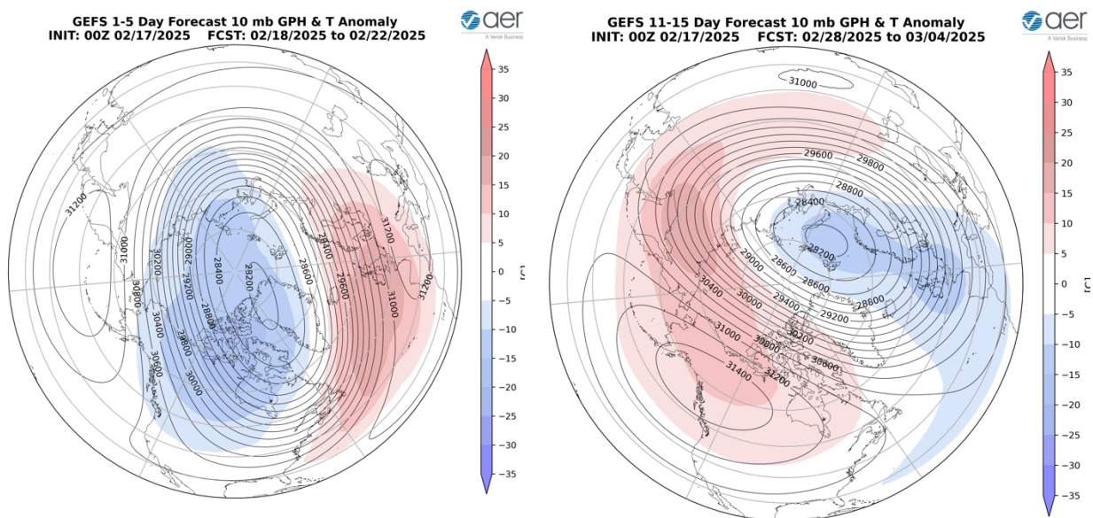
Figure 13. (a) Forecasted 10 mb geopotential heights (dam; contours) and temperature anomalies (°C; shading) across the Northern Hemisphere for 18 Feb to
