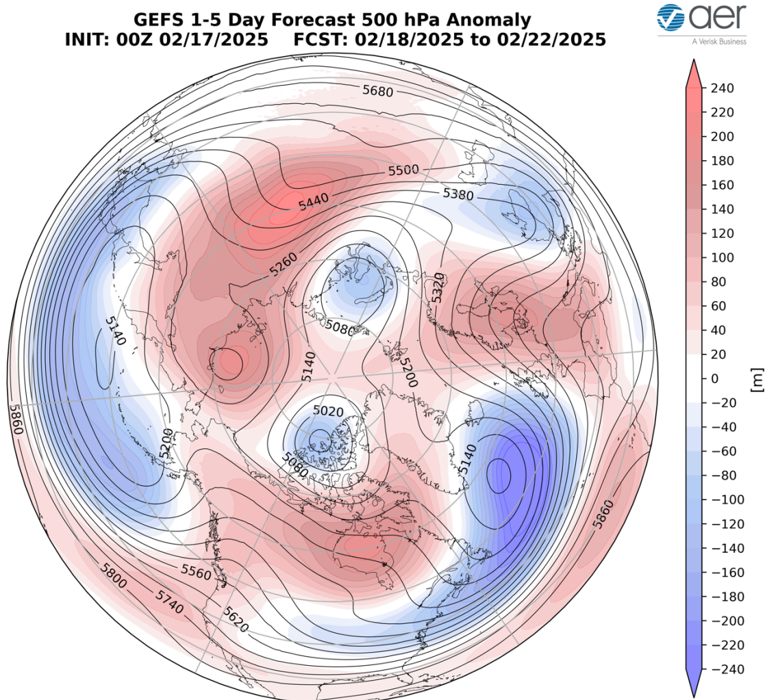
Figure 2. Forecasted average 500 mb geopotential heights (dam; contours) and geopotential height anomalies (m; shading) across the Northern Hemisphere from 18 Feb to 22 Feb 2025. The forecasts are from the 00Z 17 February 2025 GFS ensemble.
