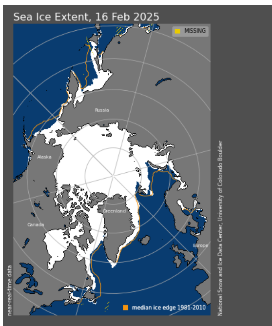
Figure 16. Observed Arctic sea ice extent on 16 February 2025 (white). Orange line shows climatological extent of sea ice based on the years 1981-2010. Image from the National Snow and Ice Data Center (NSIDC). URL: https://nsidc.org/sea-ice-today
