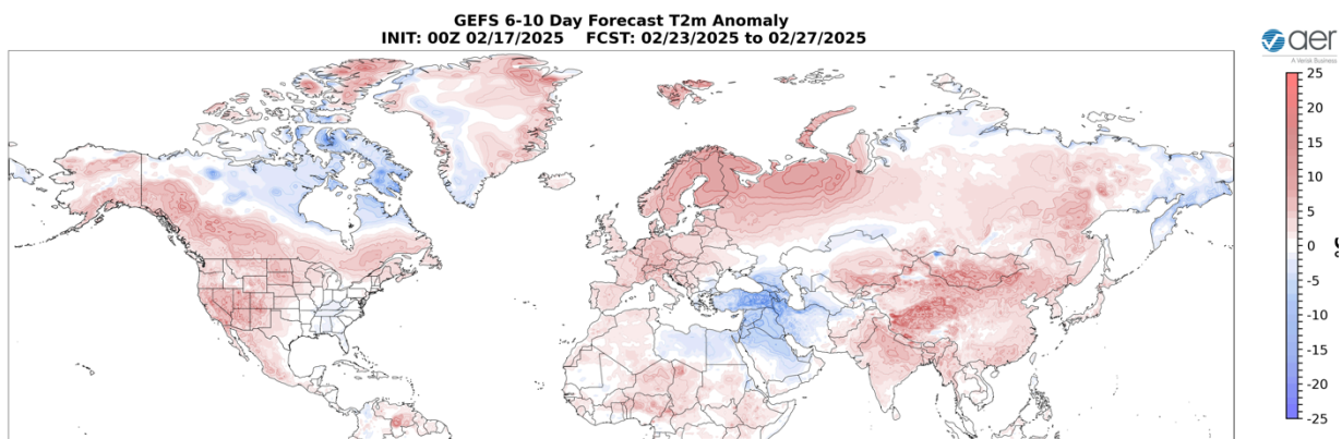
Figure 6. Forecasted surface temperature anomalies ( ^{\circ}\text{C} ; shading) from 23 Feb to 27 Feb 2025. The forecasts are from the 00Z 17 February 2025 GFS ensemble.
