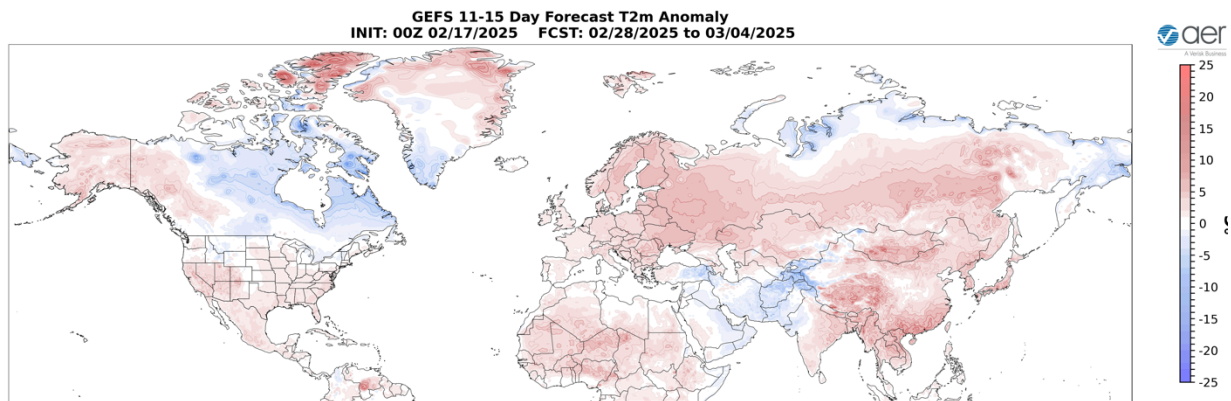
Figure 9. Forecasted surface temperature anomalies ( ^{\circ}\text{C} ; shading) from 28 Feb to 4 March 2025. The forecasts are from the 00Z 17 February 2025 GFS ensemble.
