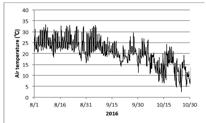
Fig. 1 Hourly temperature at Tokamachi from 1st August to 31st October of 2016
