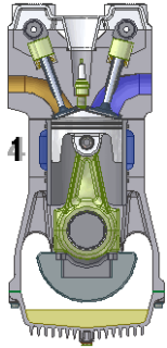
Model stroke engine
