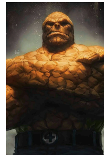
Thing (Rank 5)
