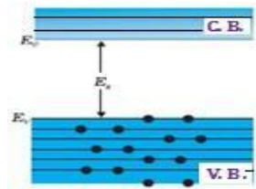
(a) at T = 0 \text{ K}
