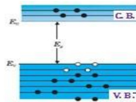
(b) at T > 0 \text{ K}
