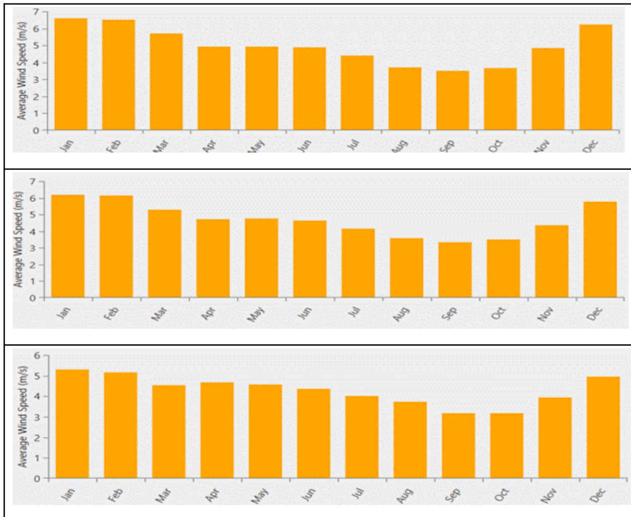
Figure 3: Annual average wind speed for Argungu, Jega and Yauri
