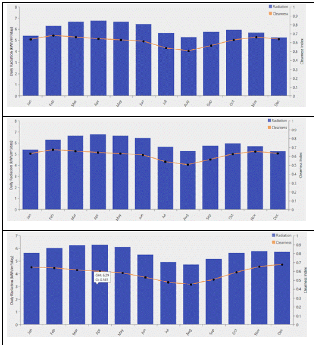
Figure 1: Annual average of solar radiation
