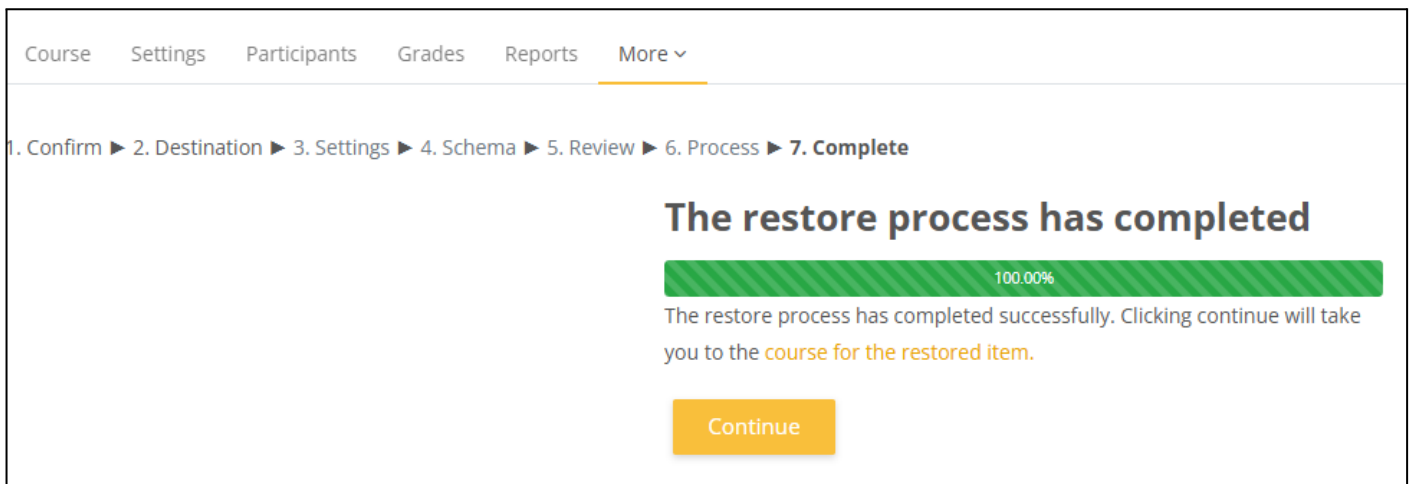
Gambar 22. Restore completed
