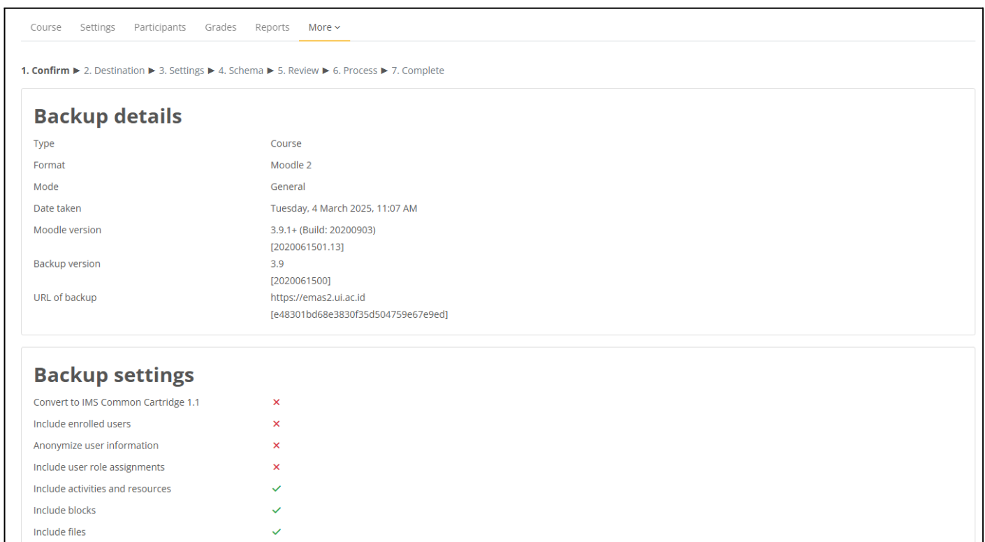
Gambar 15. Halaman Confirm
