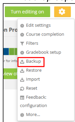
Gambar 2. Fitur Backup
