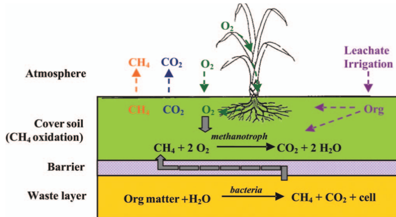
Figure 3: Microbial methane oxidation in the soil (Chiemchaisri et al., 2012)
