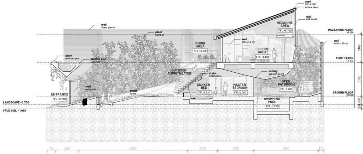
SECTION A
