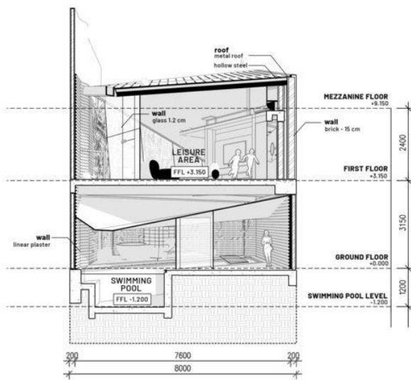
SECTION B
