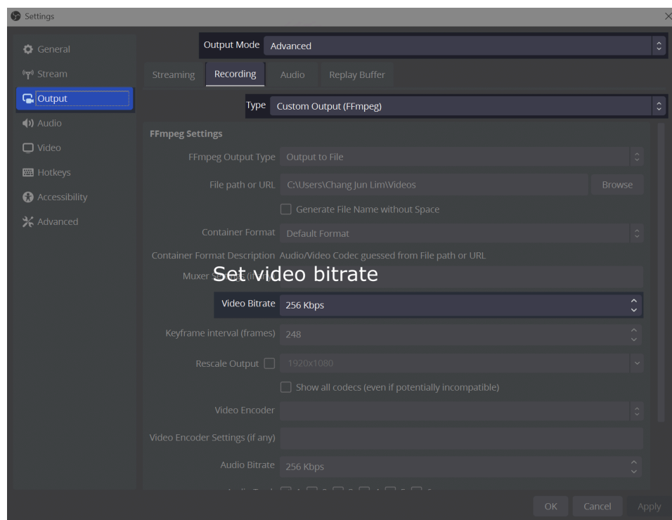
Configuration for Output
