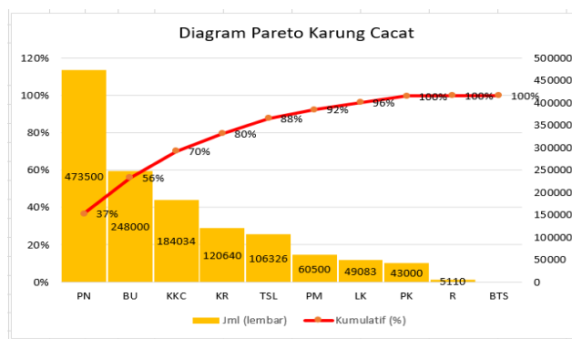
Gambar 1. Diagram Pareto
