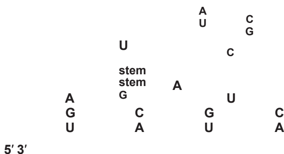
Figure 4-3 RNA Secondary Structure
