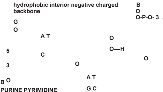
Figure 4-1 Structural Features of DNA O-P-O .
