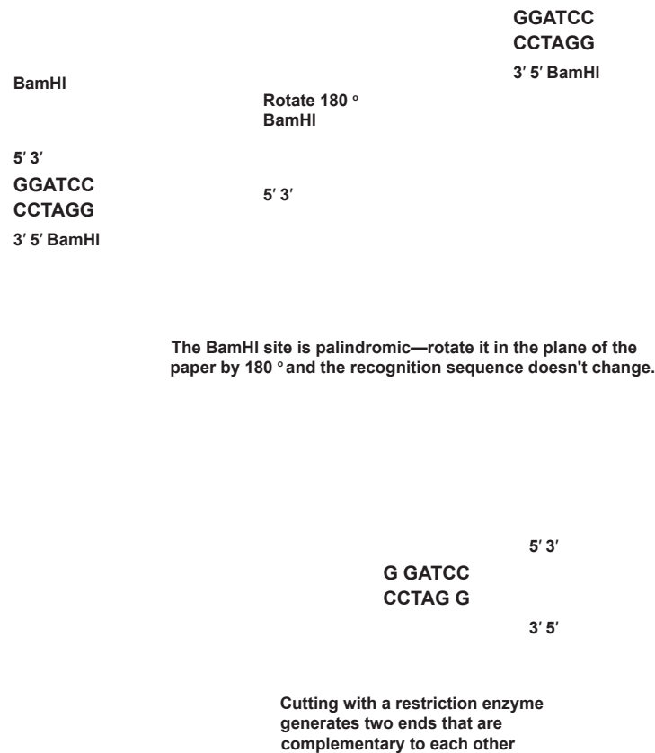
Figure 6-2 Useful RESTRICTION ENZYMES cleave DNA at symmetrical sites, leaving ends that are complementary.
