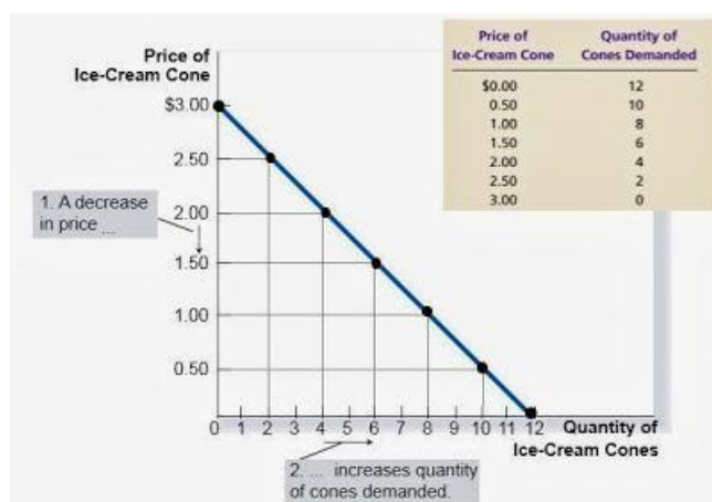
Figure 1. Statistics
