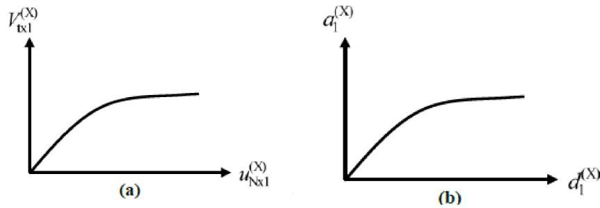
Figure 1. Cutting-displacement (a) and modal acceleration-modal displacement (b) curves (Celep, 2012).
