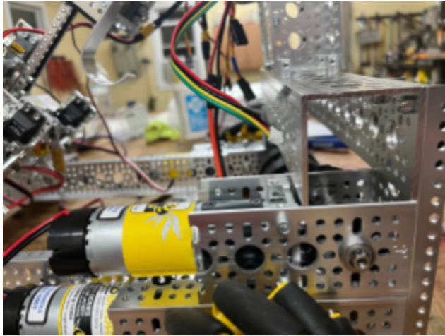
The motor we added for our intake
