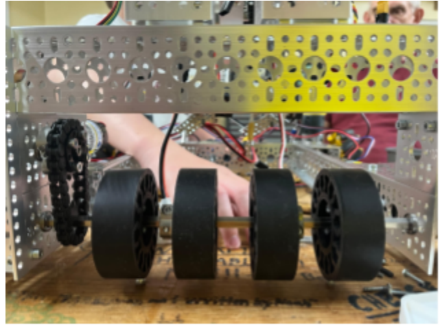
The wheels in our active intake
