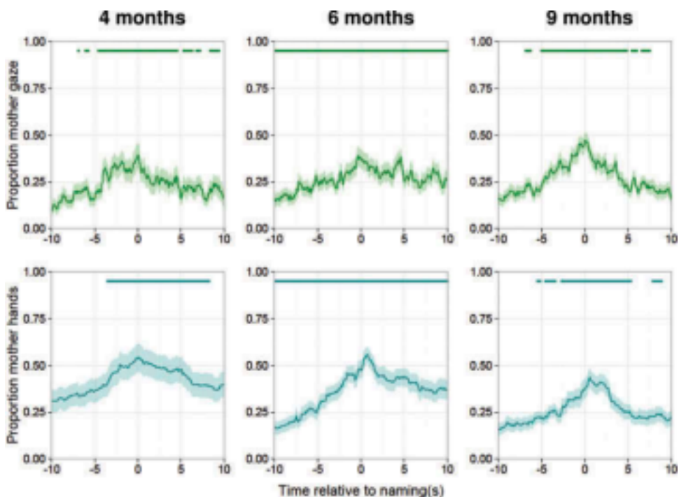
Figure 5. Mother behavior around naming utterances at each month. Lines represent average proportions of instances in which, at that time, mothers' hands or gaze were focused on the target object, time-locked to onsets of her naming utterances. Shaded regions represent the standard error of the mean. Bars at the top of graphs represent times when the naming-association index was greater than chance at p < .05 .
