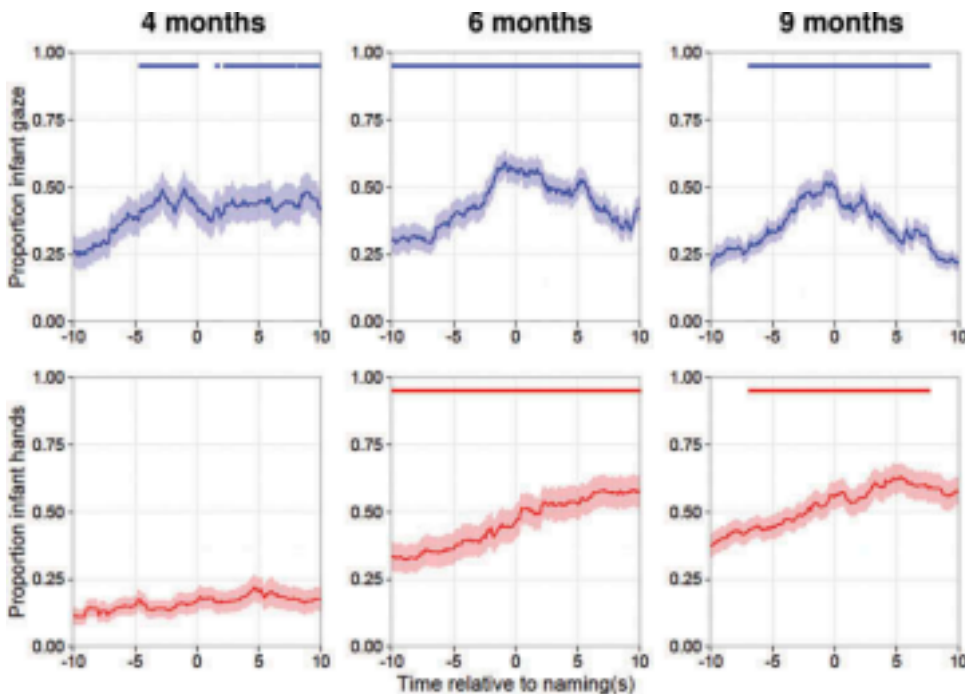
Figure 4. Infant behavior around naming utterances at each month. Lines represent average proportions of instances in which, at that time, infants' hands or gaze were focused on the target object, time-locked to onsets of naming utterances. Shaded regions represent the standard error of the mean. Bars at the top of graphs represent times when the naming-association index was greater than chance at p < .05 . 350 L. CHANG ET AL.
