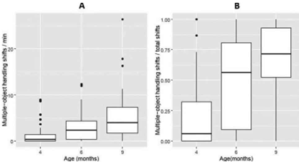
Figure 3. Increase in multiple-object handling shifts with age. A: multiple-object handling shifts per minute at each age. B: multiple-object handling shifts as a proportion of total shifts at each age.
