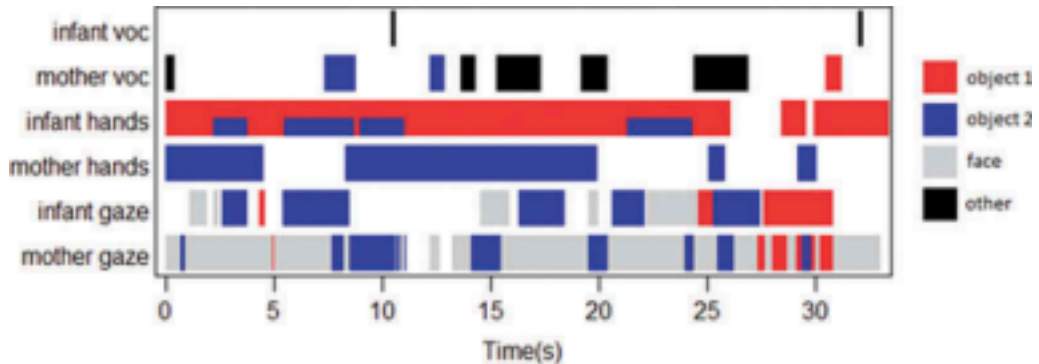
Figure 2. Example time series of data from part of one session. First row: Bars represent times when the infant vocalized. Second row: Bars represent times when the mother was speaking, and colors indicate naming utterances for the respective objects. Remaining rows: Colored bars represent times when the modality was directed to a specific target (objects or partner's face). Portions of bars split into two colors represent periods of simultaneous contact with multiple objects.
