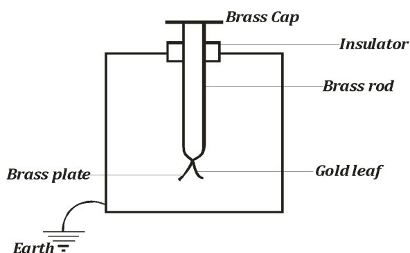
Fig. 2.1 Gold-leaf electroscope
