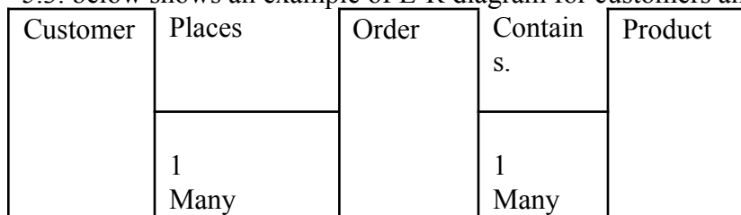
Fig. 5.3: Entity relationship diagram
