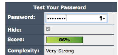
Password Meter
