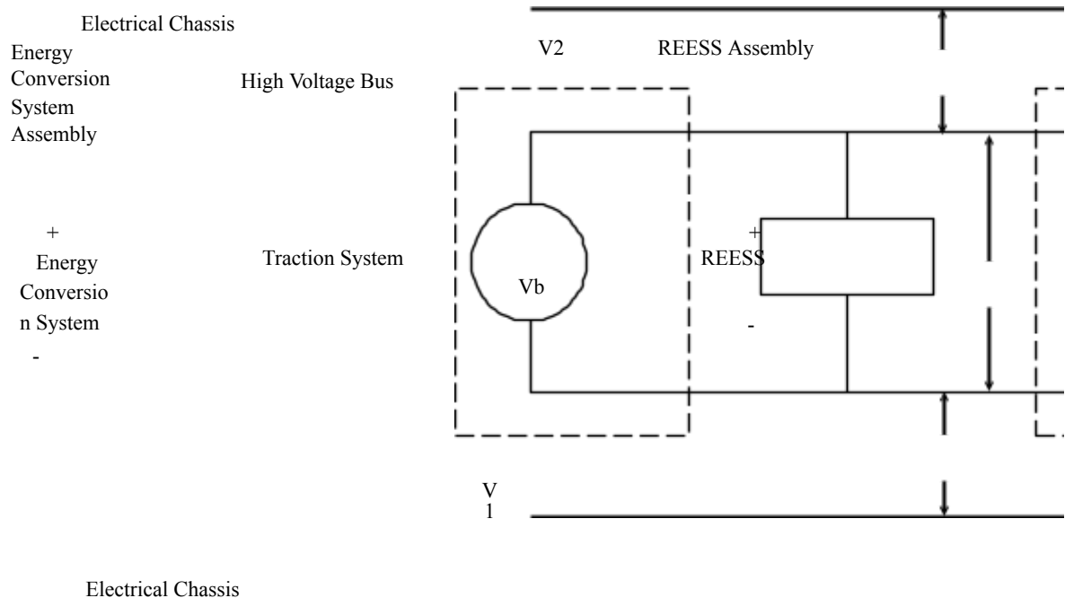
Figure 1 Measurement of V_b , V_1 , V_2
