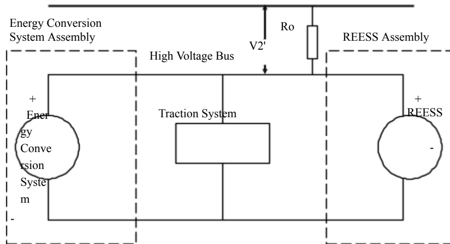
Figure 3 Measurement of V_2' Electrical Chassis
