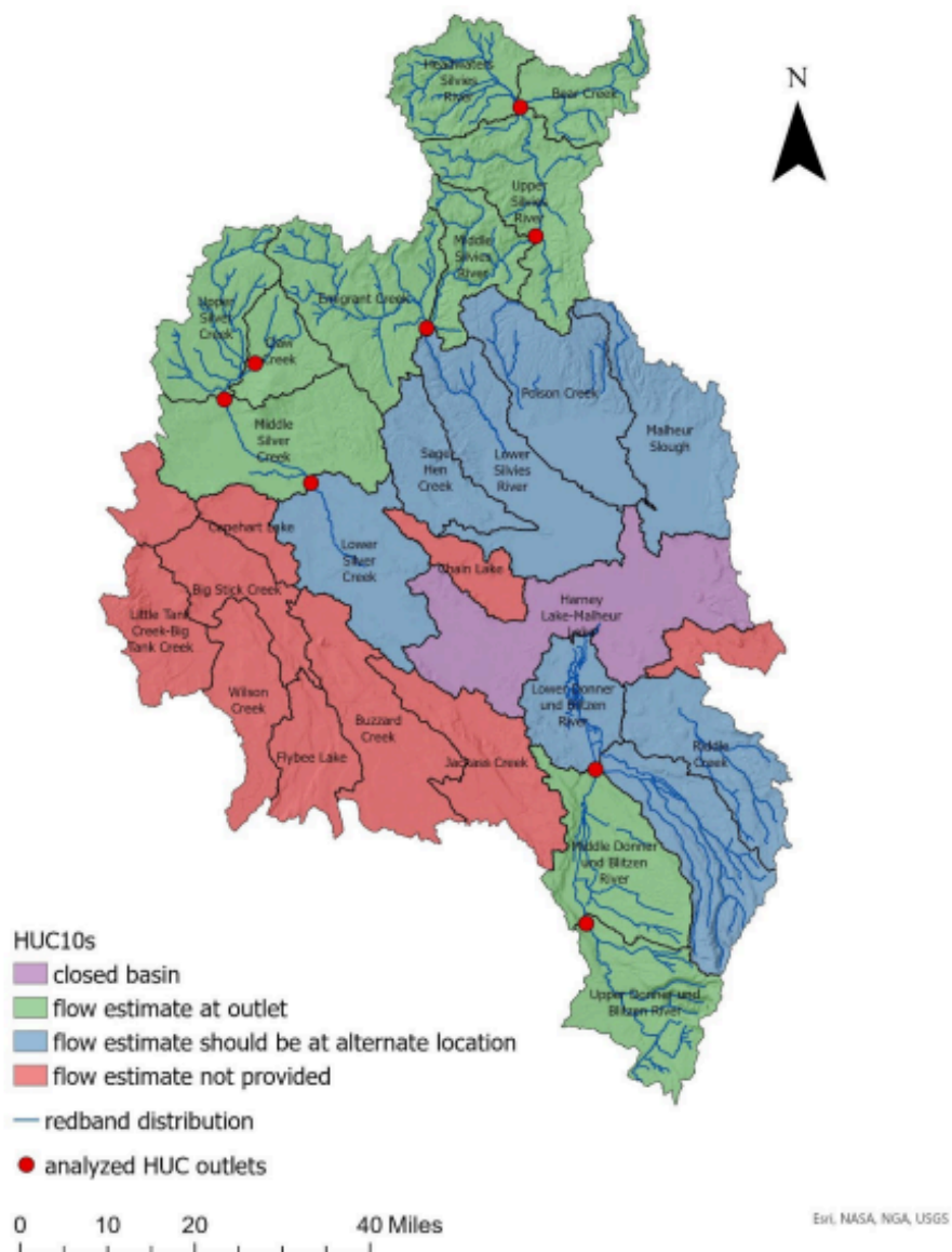
Figure 22. Map showing additional natural flow analysis locations (ODFW, 2023).
