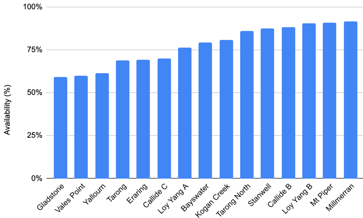
Figure 1: Availability by power station October 2025 - February 2026
