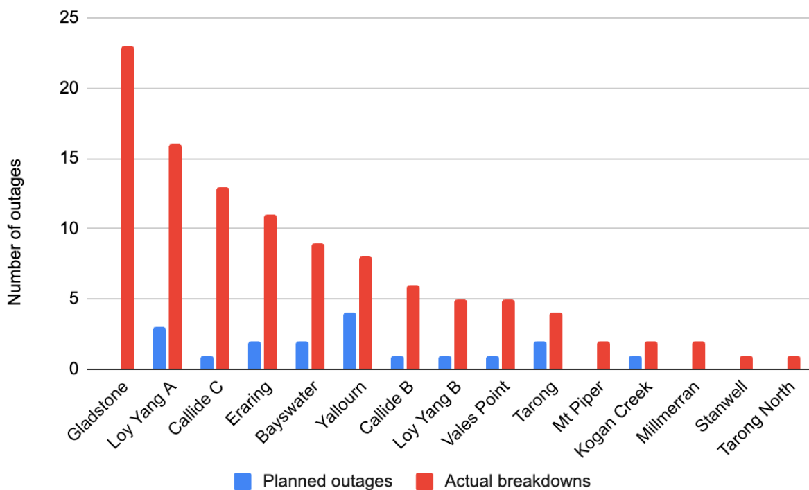
Figure 6: Planned outages vs actual breakdowns April 2025 - September 2025
