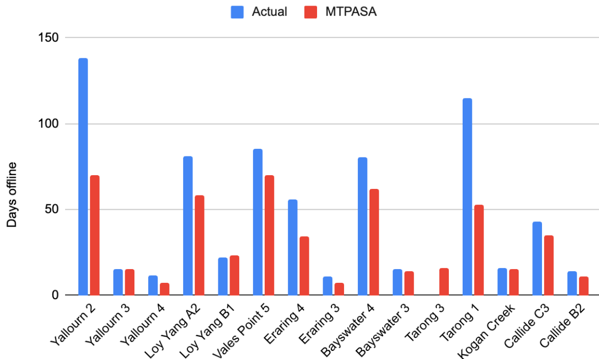
Figure 4: Maintenance overruns between October 2025 and February 2026
