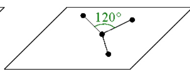
AX_3E_0 trigonal plan
