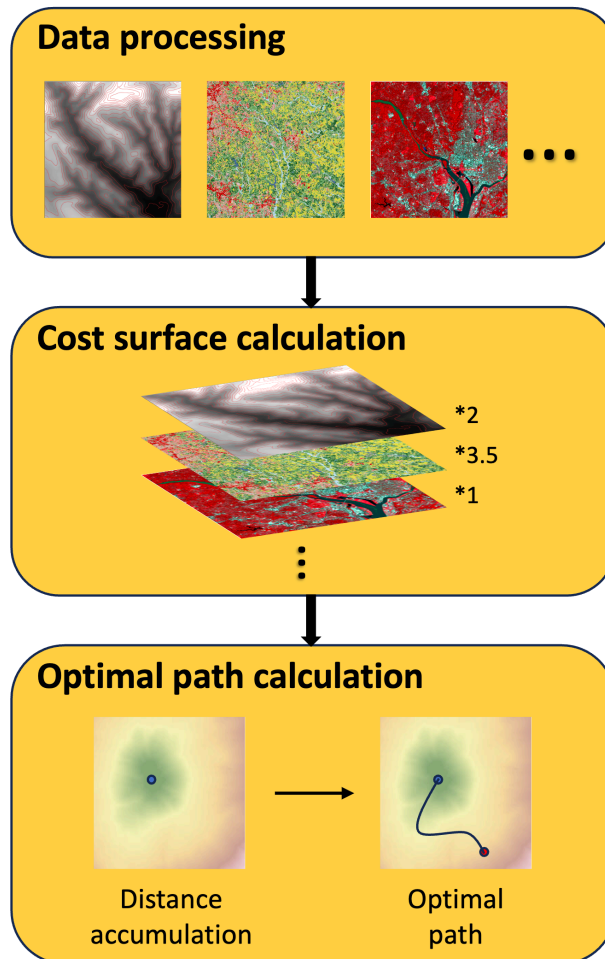
Figure 2: Optimal path calculation flowchart
