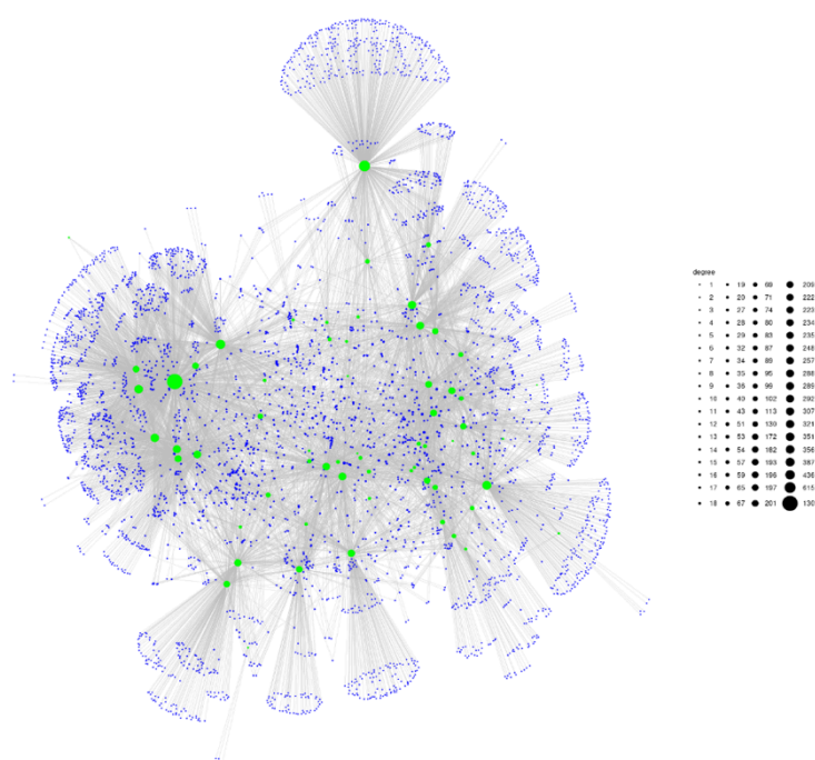
Fig.1 A bipartite network diagram, with 57 green nodes representing different paragenetic modes linked to 5659 different mineral species. Each mineral is linked to one or more paragenetic modes, while each paragenetic mode is linked to multiple minerals. There are ~12,000 links (edges) that show which minerals form by which processes.
