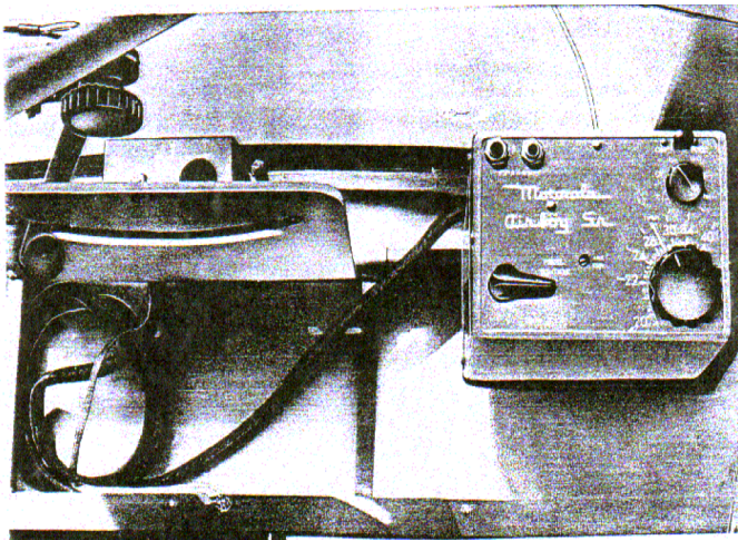
Figure 4-1. Receiver-Transmitter Set, Model L-16B
