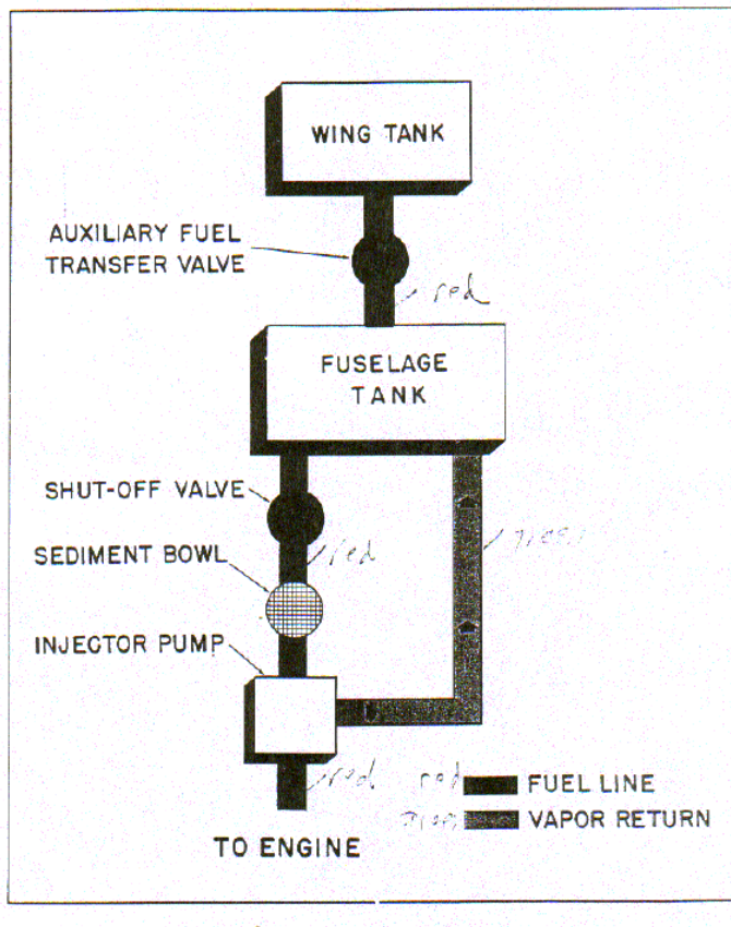
Figure 1-6. Fuel System Diagram, Model L-16B.
