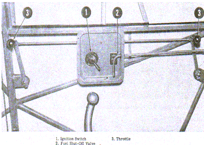
Figure 1-4. Pilot's Compartment, Left Side
