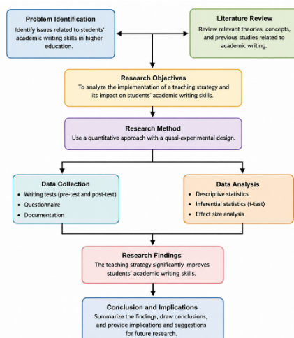
Figure 1. Research Framework
