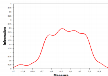
Gambar 1. Test Information Function
