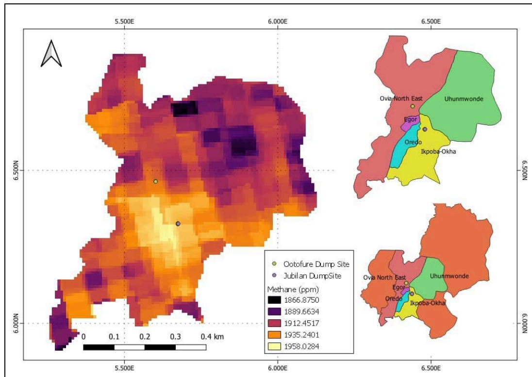
Fig.4 Spatial distribution of methane concentrations across Edo State (ppm): Emphasis on sampled dumpsites
