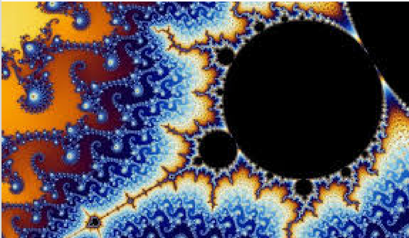
Fractal image from the Mandelbrot set
