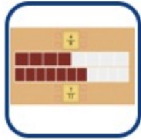
Fraction Equivalence
