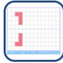
Interactive Symmetry
