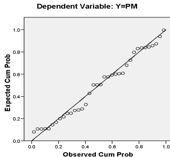
Figure 1. Normality test result
