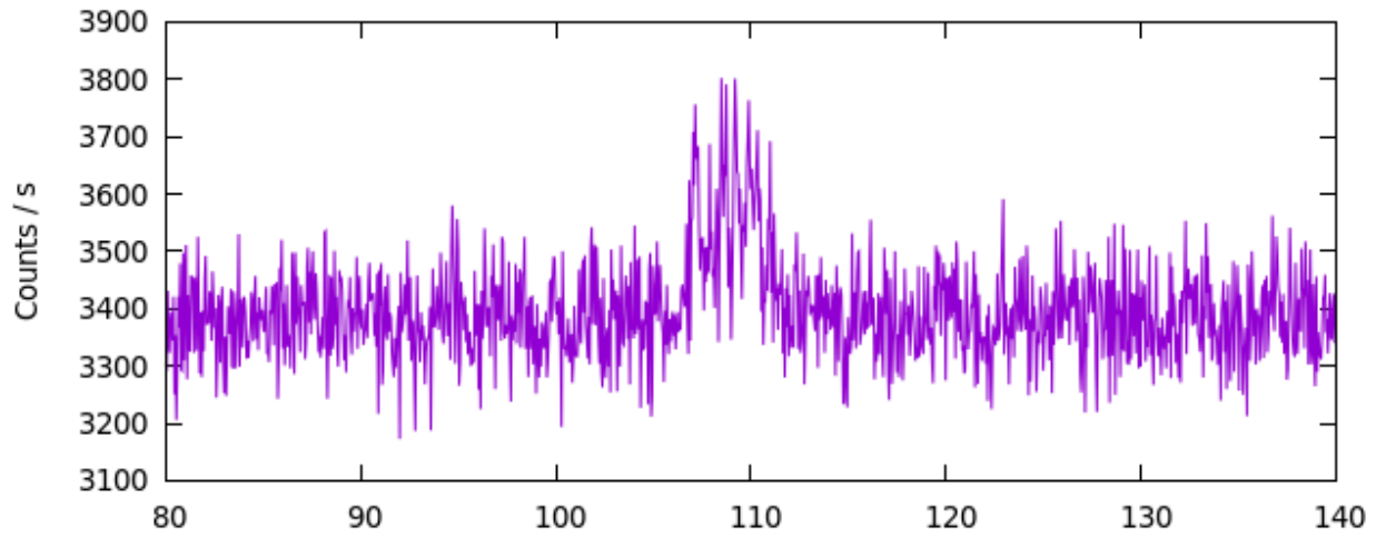
GRB 240918B : INTEGRAL SPI ACS lightcurve (0.05 s time resolution)
