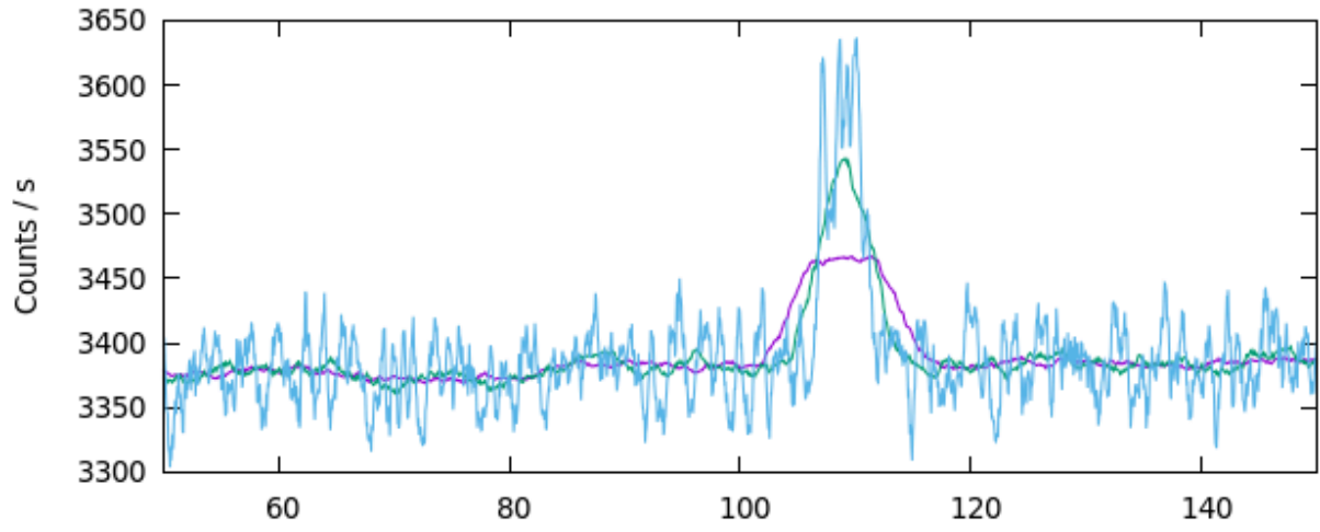
GRB 240918B : INTEGRAL SPI ACS lightcurve (10 s, 5 s, 0.5 s, running average)
