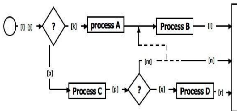
🔧 Figure 2.14: Double Link Marker Instrumentation.
