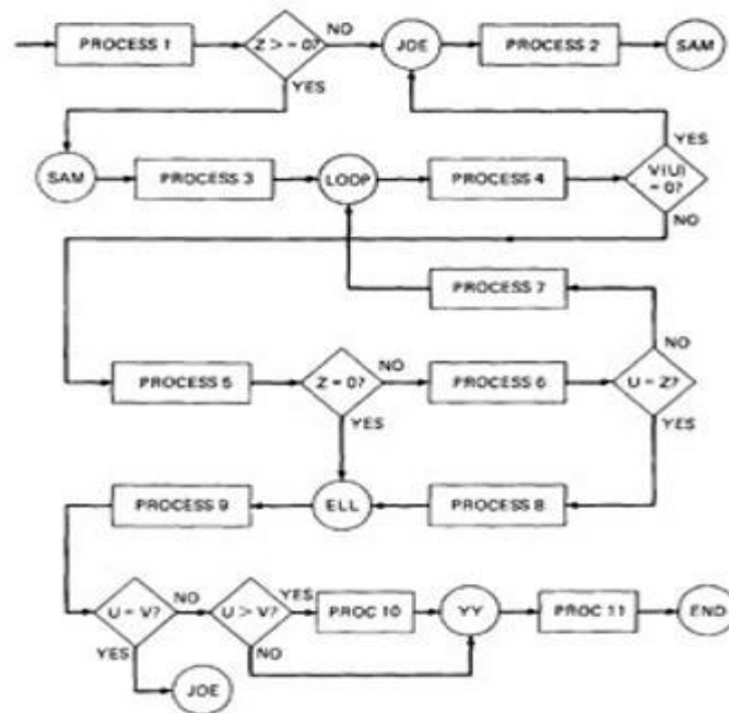
Figure 2.3: One-to-one flowchart for example program in Figure 2.2
