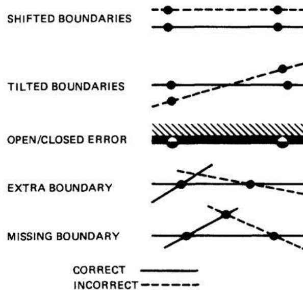
Figure 4.12: Generic Domain Bugs.
