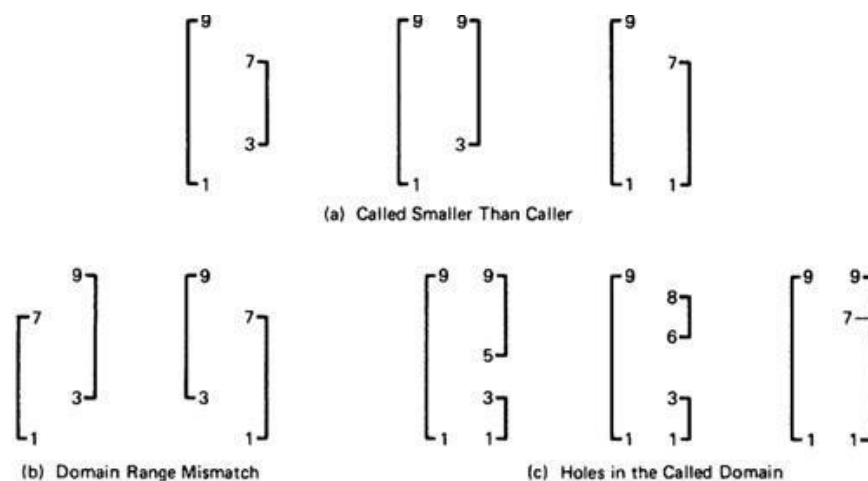
Figure 4.19: Buggy Range / Domain Mismatches
