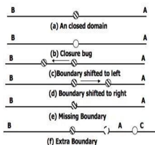
Figure 4.14: One Dimensional Domain Bugs, Closed Boundaries.
