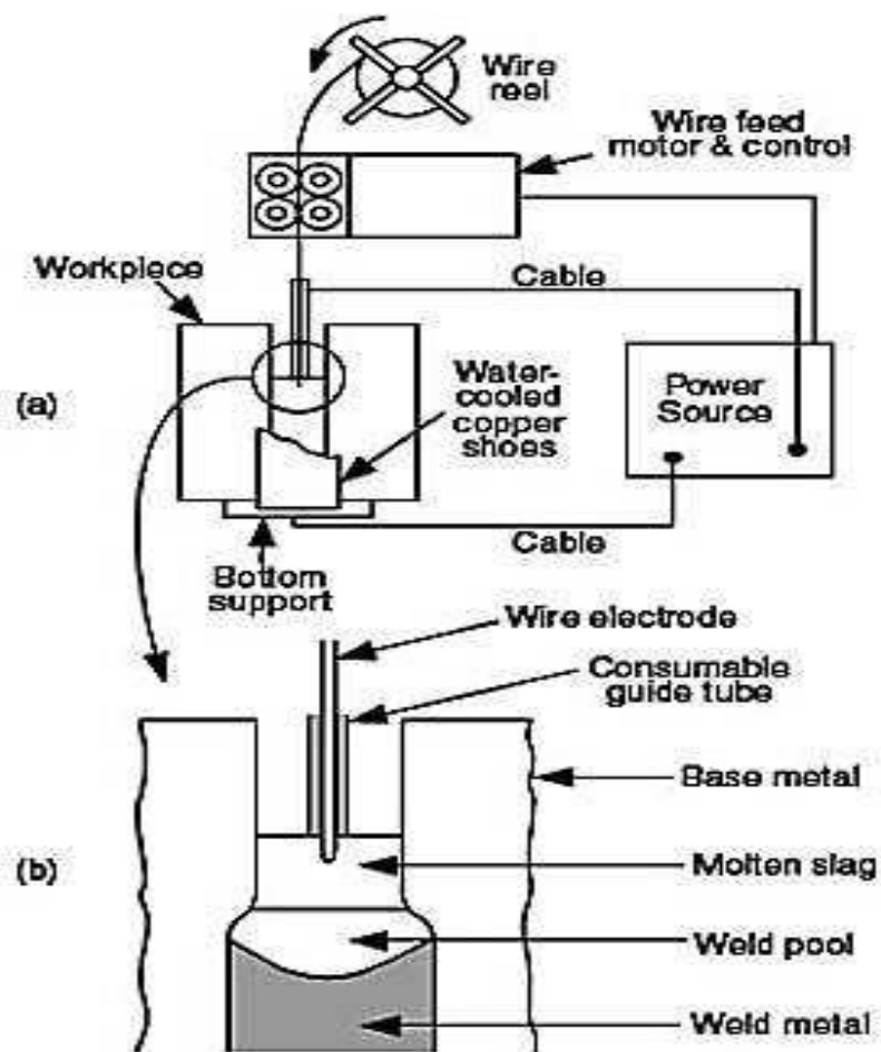
Fig.2.9 Electroslag welding
