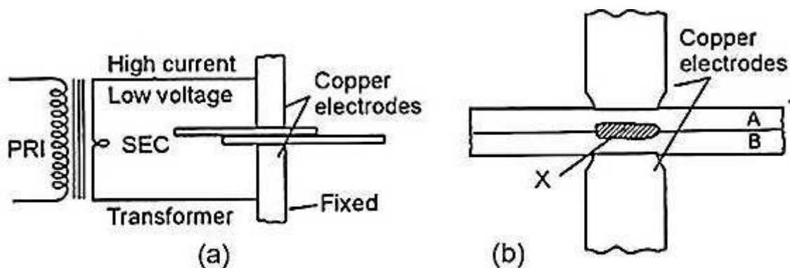
Fig. 2.12 : Spot Welding
