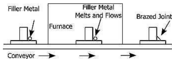
Fig.2.23 Furnace Brazing
