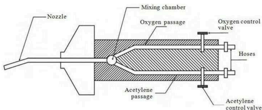
Fig.2.3 Welding Torch
