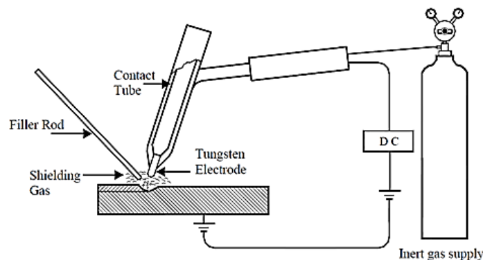
Fig.2.6 Gas Tungsten Arc Welding
