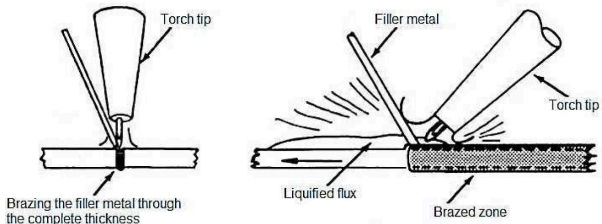
Fig.2.22 Brazing Process
