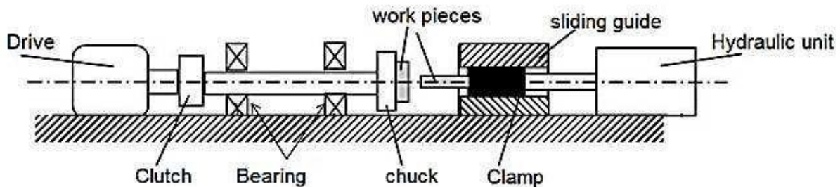
Fig.2.20 : Friction Welding
