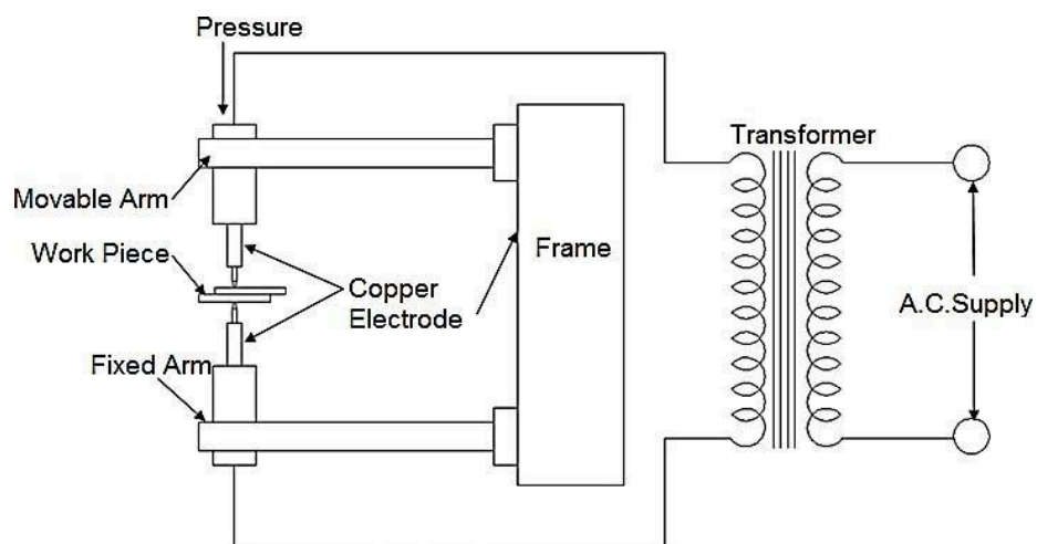
Fig. 2.10 : Resistance welding
