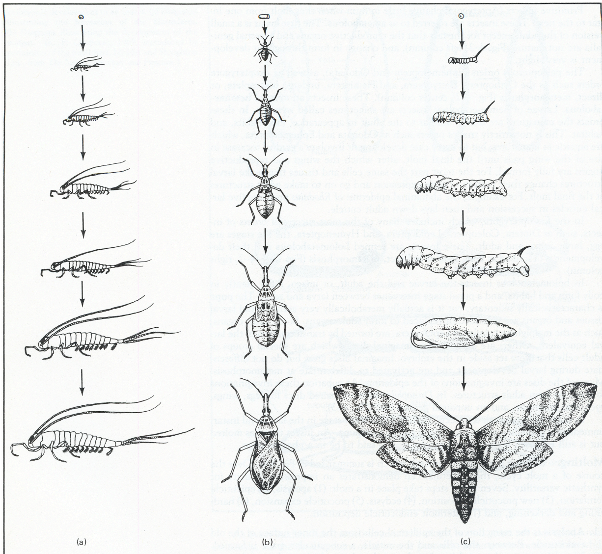
Figure 4-2 Basic types of development in insects. (a) Machilis (Archeognatha); (b) Rhodnius (Hemiptera); (c) Manduca (Lepidoptera).
