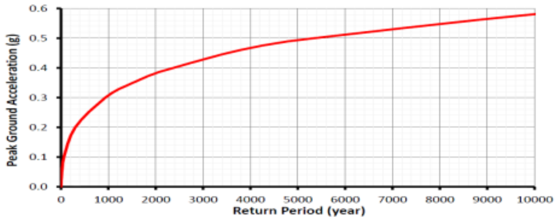
Gambar 3 Hazard PGA Vs Periode ulang
